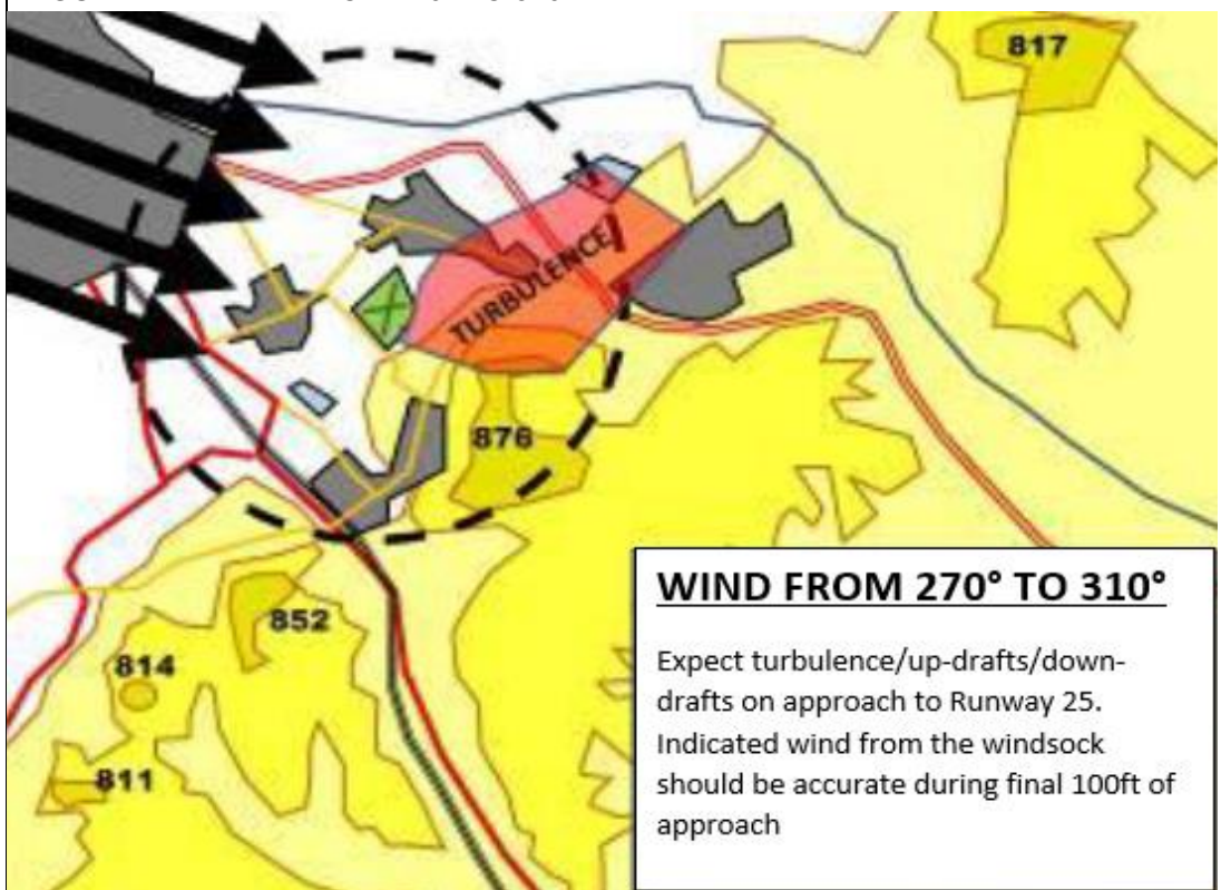
FIGURE 4 – WINDS FROM 270° TO 310°
