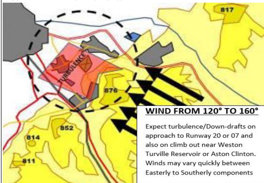
FIGURE 2 – WINDS FROM 120° TO 160°
